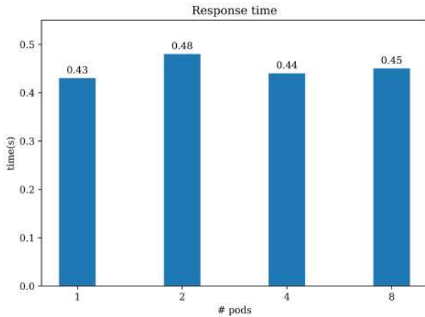
Figure 6: Response Time.
