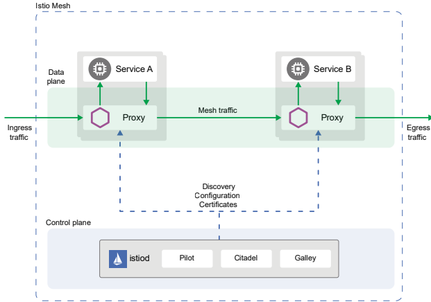
Figure 1: Istio Architecture [10].
