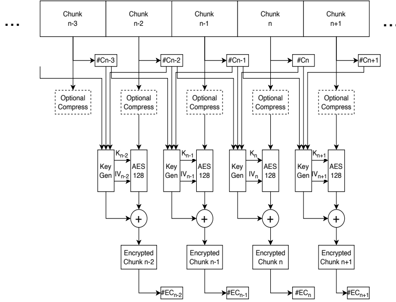
Fig. 1: Self-encryption process, adopted from [11]
