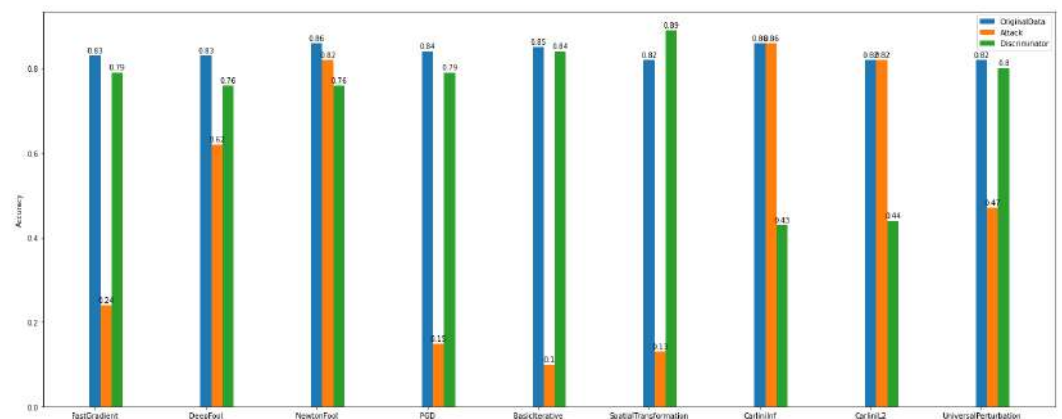
Figure 23. Multi-class discriminator—Dataset_2.
