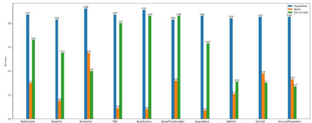
Figure 22. Multi-class discriminator—Dataset_1.
