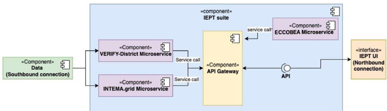
Figure 4. Component diagram of the IEPT suite.
