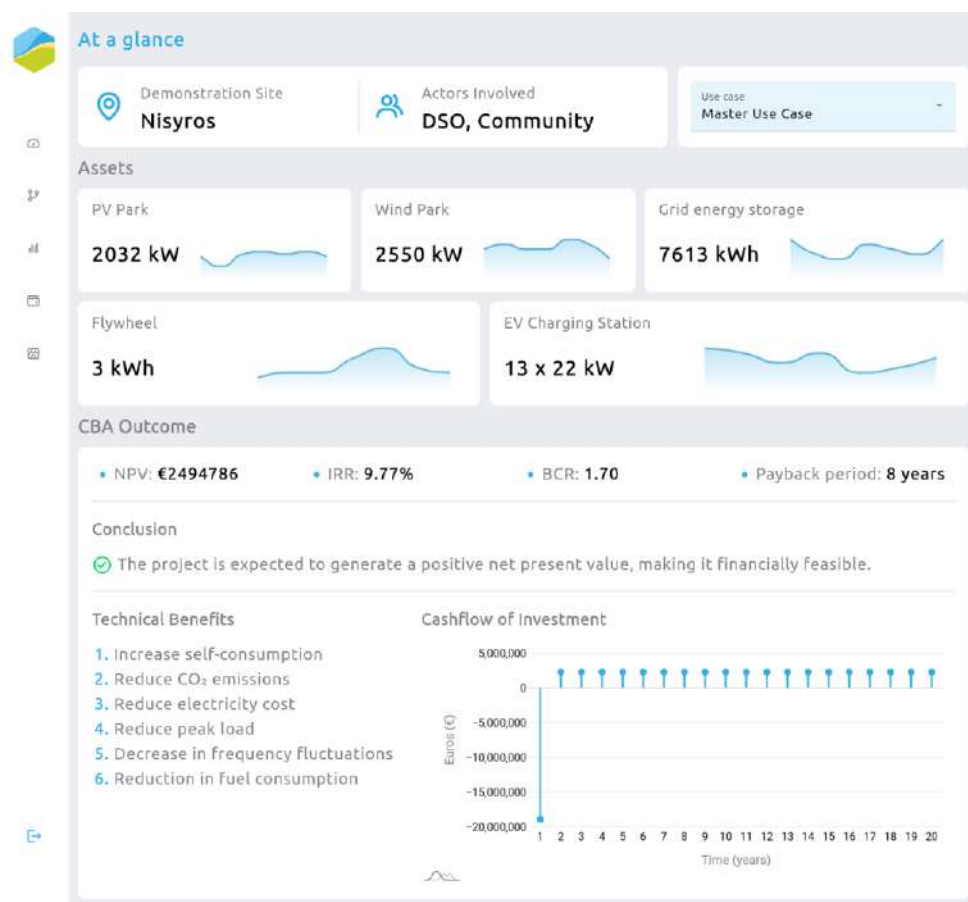
Figure 5. The “at-a-glance” page of the IEPT dashboard with the results of the CBA module.
